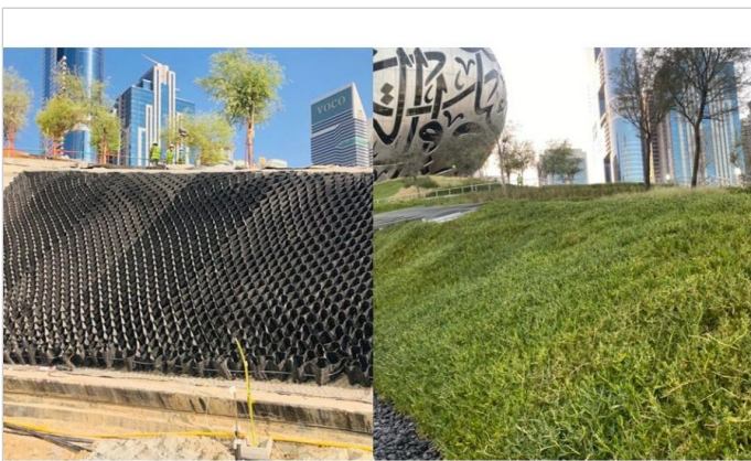
During construction: Macweb geocell (before & after vegetation growth)
