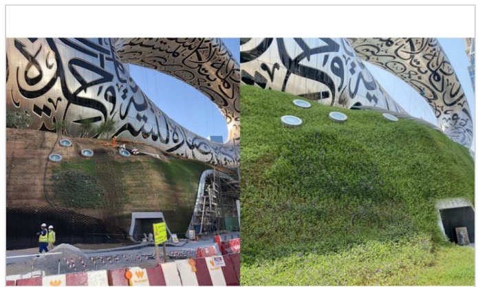
During construction: Green Terramesh soil slope (before & after vegetation)
