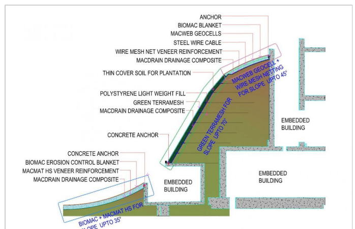
Sectional detail of Maccaferri green cover solutions
