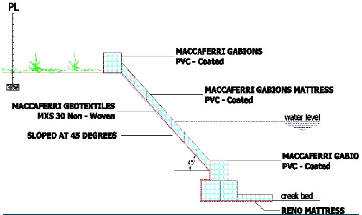
Proposed Section
