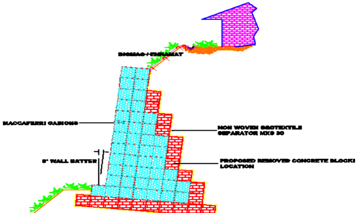
Proposed Section
